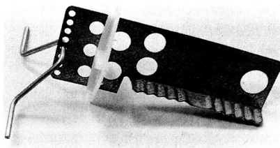
Adjustable rigid tie with wire component for brick wythe
