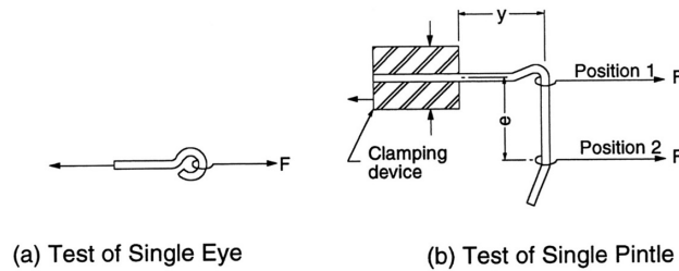
Figure 13.12 Effect of adjustability on capacity of pintle ties (from Ref. 13.11).
