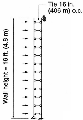
(a) Wall Configuration
